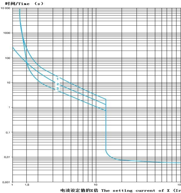
NDD1-32 current/time characteristic curve 20±2℃
